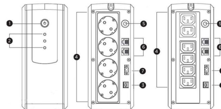
UT1200EG / UT1200EIG (Schuko / IEC Outlet)
