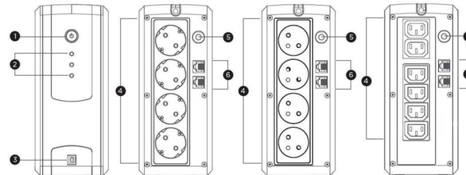
UT1050EG / UT1050EIG (Schuko / French / IEC Outlet)
